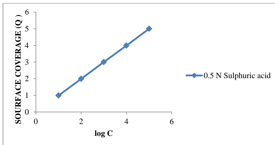
Figure 10: Temkin adsorption isotherm plot for zinc in 0.5N H 2 SO 4 containing different concentrations of the inhibitor.
