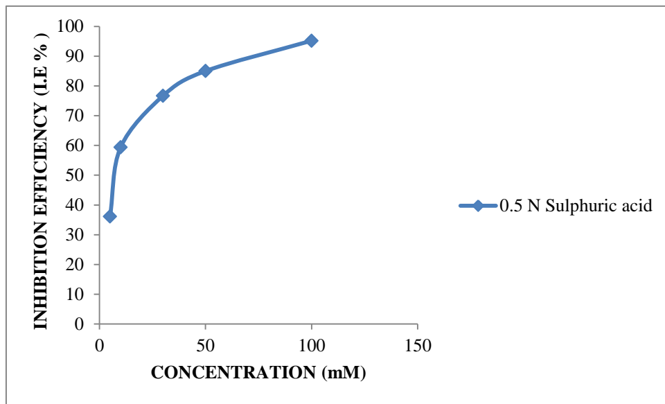
Figure 3: Variation of inhibition efficiency with concentration of the 2-Mercapto -1- Methyl imidazole inhibitor for zinc in 0.5 N H_2SO_4
