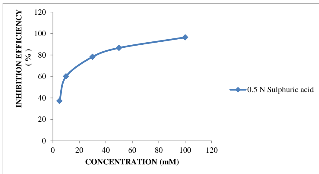
Figure 5: Variation of inhibition efficiency with concentration of the 2-Mercapto -1- Methyl imidazole inhibitor for zinc in 0.5 N H 2 SO 4
