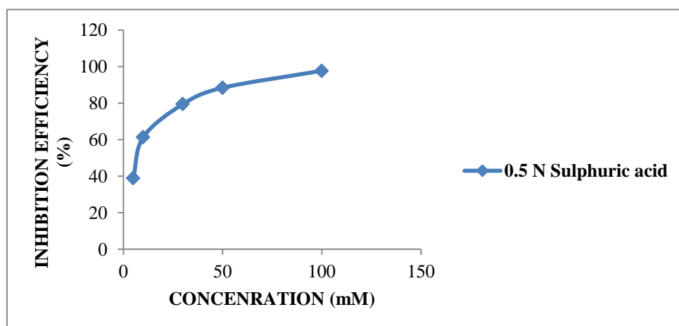
Figure 1: Variation of inhibition efficiency with concentration of the 2-Mercapto -1- Methyl imidazole inhibitor for zinc in 0.5 N H 2 SO 4
