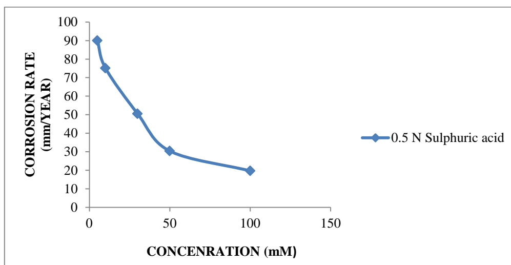
Figure 2: Variation of corrosion rates with concentration of the the 2-Mercapto -1Methyl imidazole inhibitor for zinc in 0.5 N H_2SO_4
