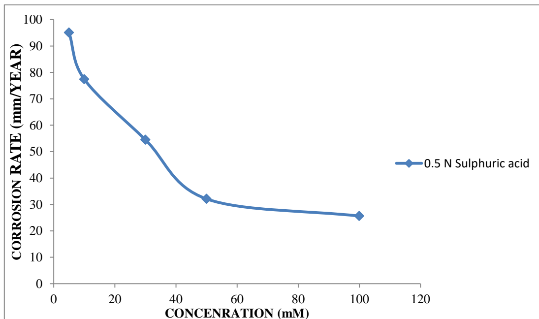
Figure 4: Variation of corrosion rates with concentration of the the 2-Mercapto -1Methyl imidazole inhibitor for zinc in 0.5 N H_2SO_4
