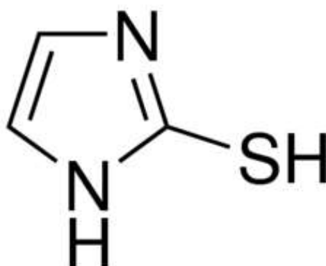
Figure 7: The structure of the 2-Mercapto -1Methyl imidazole
