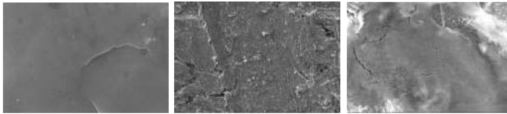
Fig 8: Scanning electron micrographs of zinc immersed for 30 minutes (a) polished Zinc (b) zinc metal immersed in 0.5 N H 2 SO 4 (c) zinc metal immersed in 0.5 N H 2 SO 4 with 2-Mercapto -1Methyl imidazole
