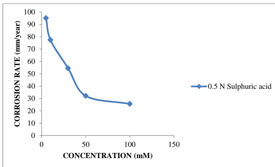
Figure 6: Variation of corrosion rates with concentration of the the 2-Mercapto -1Methyl imidazole inhibitor for zinc in 0.5 N H 2 SO 4
